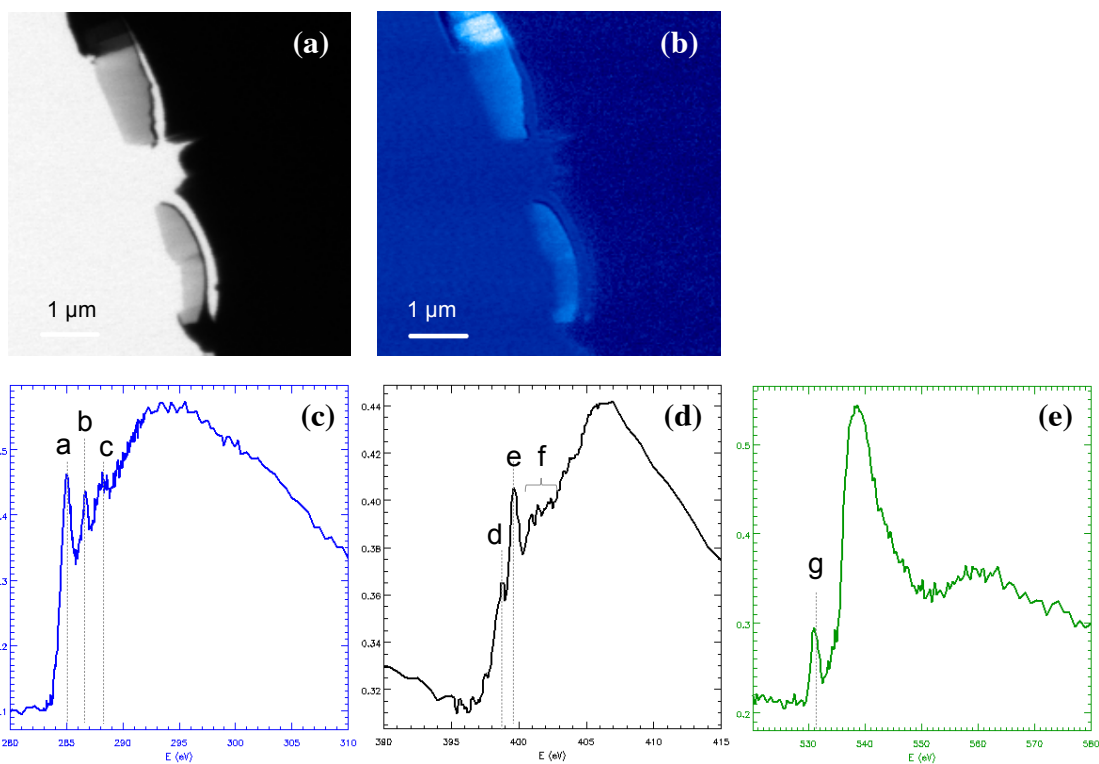
Fig. 1. (a) Scanning transmission x-ray microscope (STXM) image acquired at 340 eV, (b) carbon map, (c) C-XANES spectrum, (d) N-XANES spectrum, and (e) O-XANES spectrum for RB-QD04-0047-02-01. Peak a corresponds to 1s-\pi^* transition of aromatic/olefinic carbon ( C=C ) at 285.1 eV; Peak b corresponds to 1s-\pi^* transition of vinyl-keto ( C=C-C=O ), nitrile ( C\equiv N ), and/or nitrogen heterocycles ( C-N=C ) at 286.7 eV; Peak c corresponds to 1s-\pi^* transition of carboxyl carbon ( COOH ) at 288.2 eV; Peak d corresponds to 1s-\pi^* transition of imine ( C=N ) at 398.9 eV; Peak e corresponds to 1s-\pi^* transition of nitrogen heterocycles ( C-N=C ) and/or nitrile ( C\equiv N ) at 399.7 eV; Assembly of small peaks (f) is related to the 1s-\pi^* transition of amide ( R-(C=O)NR'_2 ) and the 1s-3p/s^* transitions of pyrrolic ( C_4H_4NH ) and amine ( R-NH_2 ) at 401-402.5 eV; and Peak g corresponds to 1s-\pi^* transition of ketone group ( C=O ) at 531 eV.
